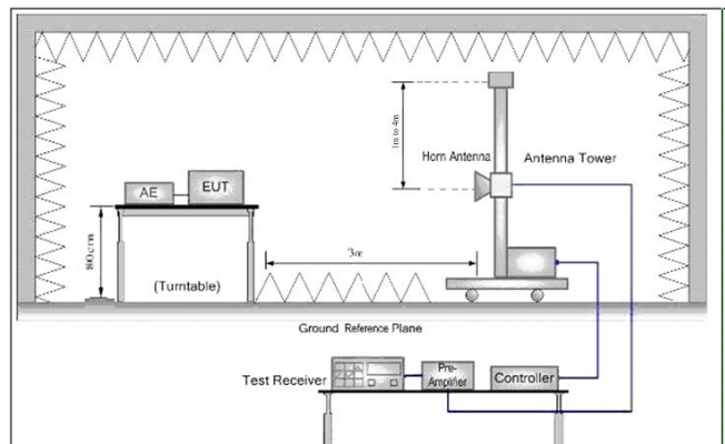
Figure 2. Above 1 GHz
